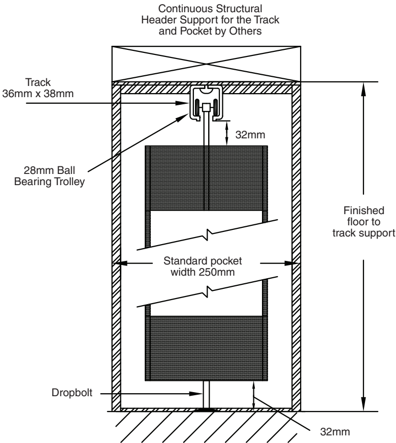
VERTICAL SECTION
